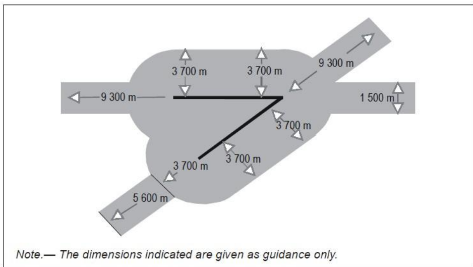
Figure 2. Multiple runway laser-beam free flight zones
