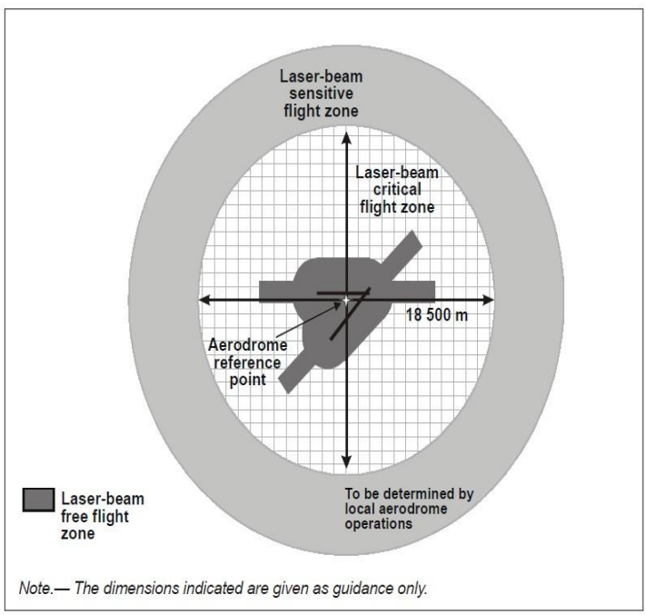
Figure 1. Protected flight zones
